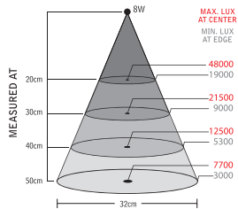
Sunmach 10 LED Light, 24V/8W, 36° Lens
